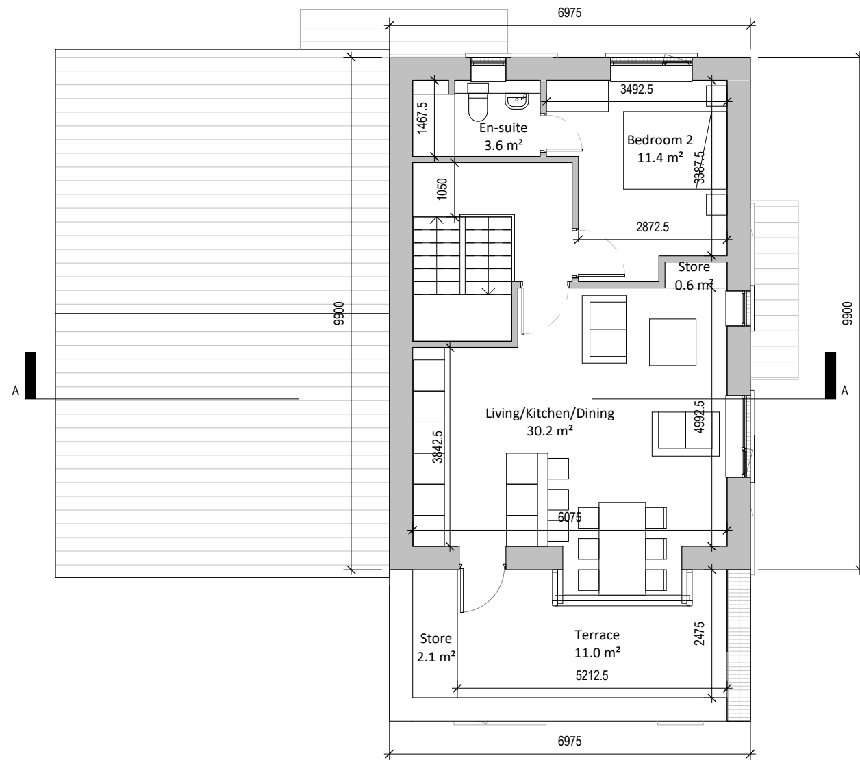
① Second Floor 1 : 100
